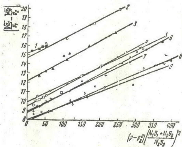
Fig. 1. 1 - \text{H}_2 - \text{C}_2\text{H}_4 ( 188.1^\circ\text{K} ); 2 - \text{H}_2 - \text{CH}_4 ( 90.3^\circ\text{K} ); 3 - \text{H}_2 - \text{CH}_4 ( 110.0^\circ\text{K} ); 4 - \text{H}_2 - \text{CO} ( 68.1^\circ\text{K} ); 5 - \text{H}_2 - \text{N}_2 ( 63.1^\circ\text{K} ); 6 - \text{H}_2 - \text{CO} ( 73.1^\circ\text{K} ); 7 - \text{H}_2 - \text{N}_2 ( 68.1^\circ\text{K} ); 8 - \text{H}_2 - \text{CO} ( 83.1^\circ\text{K} ); 9 - \text{H}_2 - \text{N}_2 ( 78.1^\circ\text{K} ).
